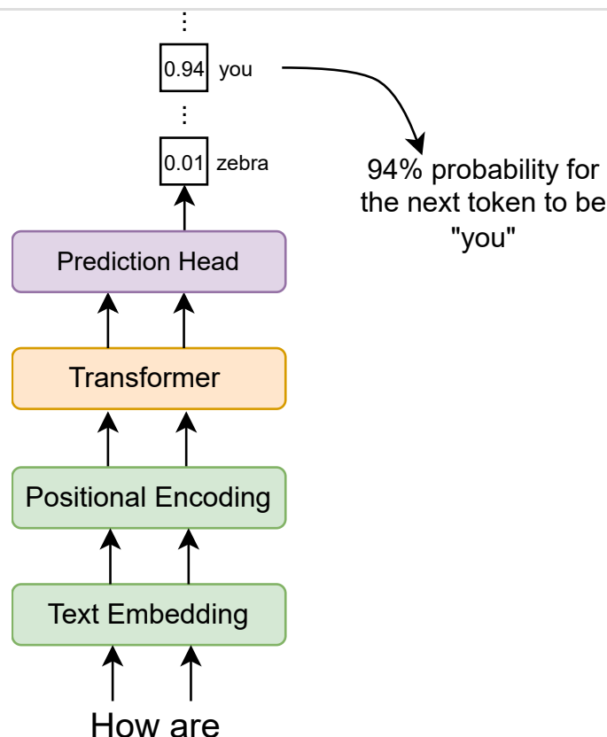
Figure 22: Prediction head output probabilities
