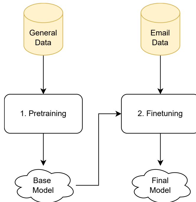
Figure 23: Two-stage training strategy
