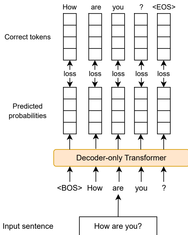
Figure 27: Parallelizing loss computations over different lengths
