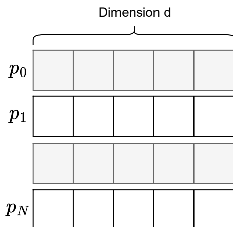
Figure 20: Trainable matrix representing positional encodings
