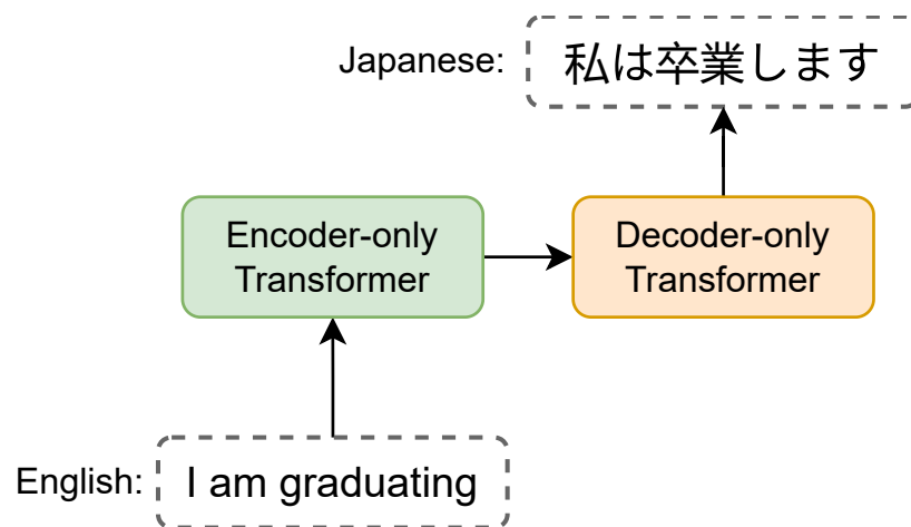
Figure 13: Encoder-decoder Transformer used for language translation
