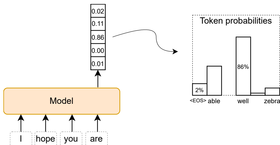
Figure 24: Probability distribution in next-token prediction
