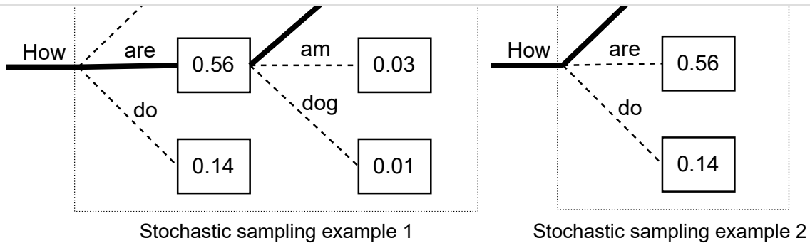
Figure 35: Stochastic sampling randomness
