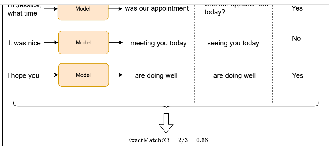
Figure 39: Example of calculating ExactMatch@3 for three sequences
