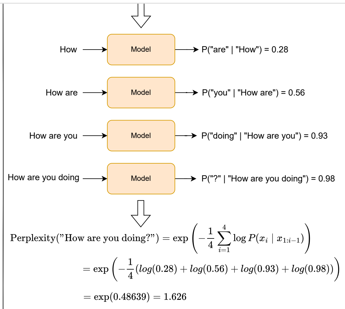
Figure 38: Example of perplexity calculation
