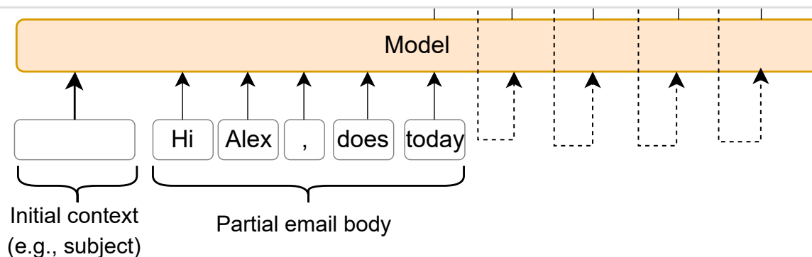
Figure 32: Sampling email completion token by token
