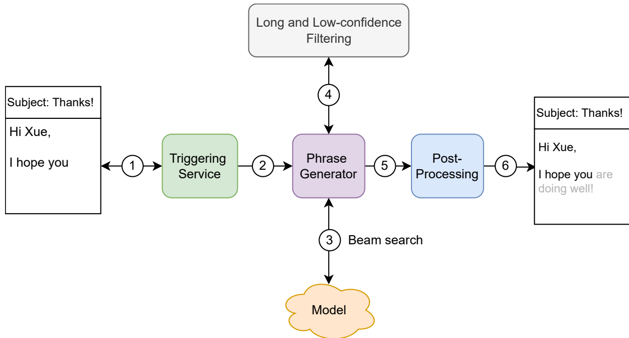
Figure 43: Smart Compose feature overall design
