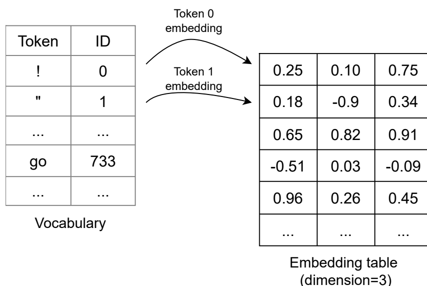
Figure 15: Embedding table representing tokens
