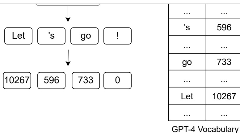
Figure 10: Example of token indexing
